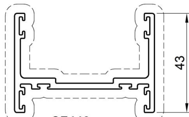
CF446 GUIDE / RECEIVER
