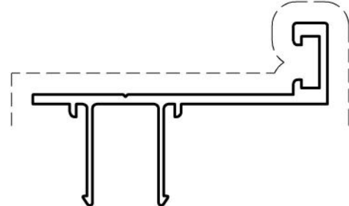
CF107 45mm DOOR STOP
