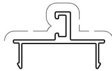
RC413 45mm DOOR STOP - 101.6mm DG (36mm POCKET)
