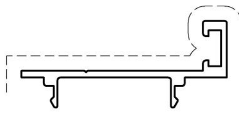
DG107 45mm DOOR STOP
