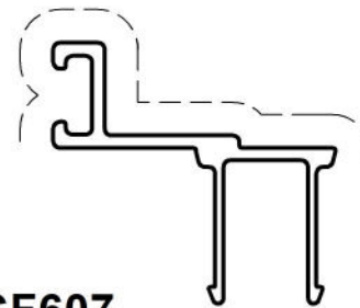
CF607 45mm DOOR STOP SG CENTRE GLAZED
