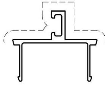
CF707 45mm DOOR STOP - 101.6mm DG
