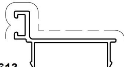
RC613 45mm DG DOOR STOP - 150mm DG (36mm POCKET)
