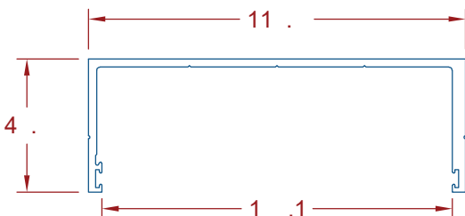
CF477 - Heavy Duty Subhead (113mm x 40mm)
