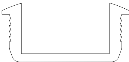
CFH29 - 24mm-25mm Glazing Channel
