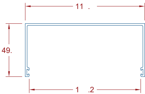
CF437 - Standard Subhead (110mm x 49mm)
