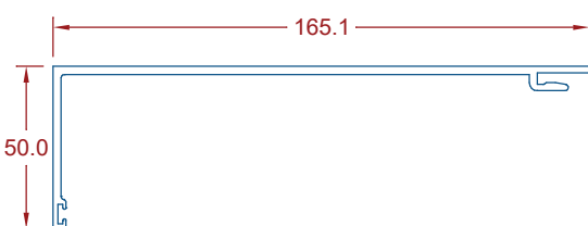
CF658 - 150mm Subhead 2 Piece
