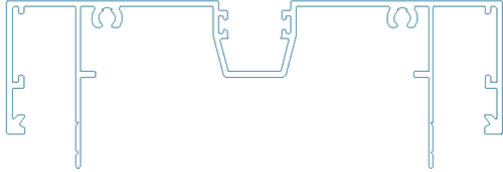
CFP 901 – Door Frame (Frame With Legs)
