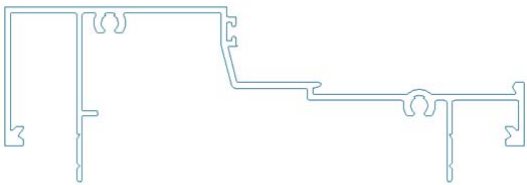
CFP 903 – Window Sill
