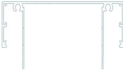
CFP 812 - Flat Ceiling Channel
