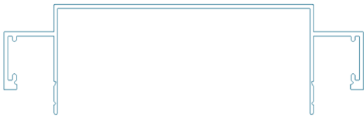
CFP 902 – Ceiling Channel (10mm Shadowline)
