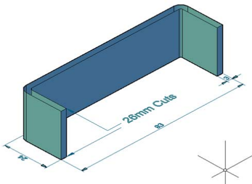
CFP 813 – Floor Guides (Mill Finish Only)
