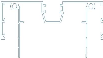
CFP 811 - Door Frame (Frame With Legs)
