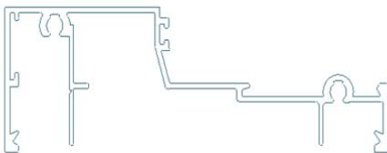
CFP 803 - Window Sill
